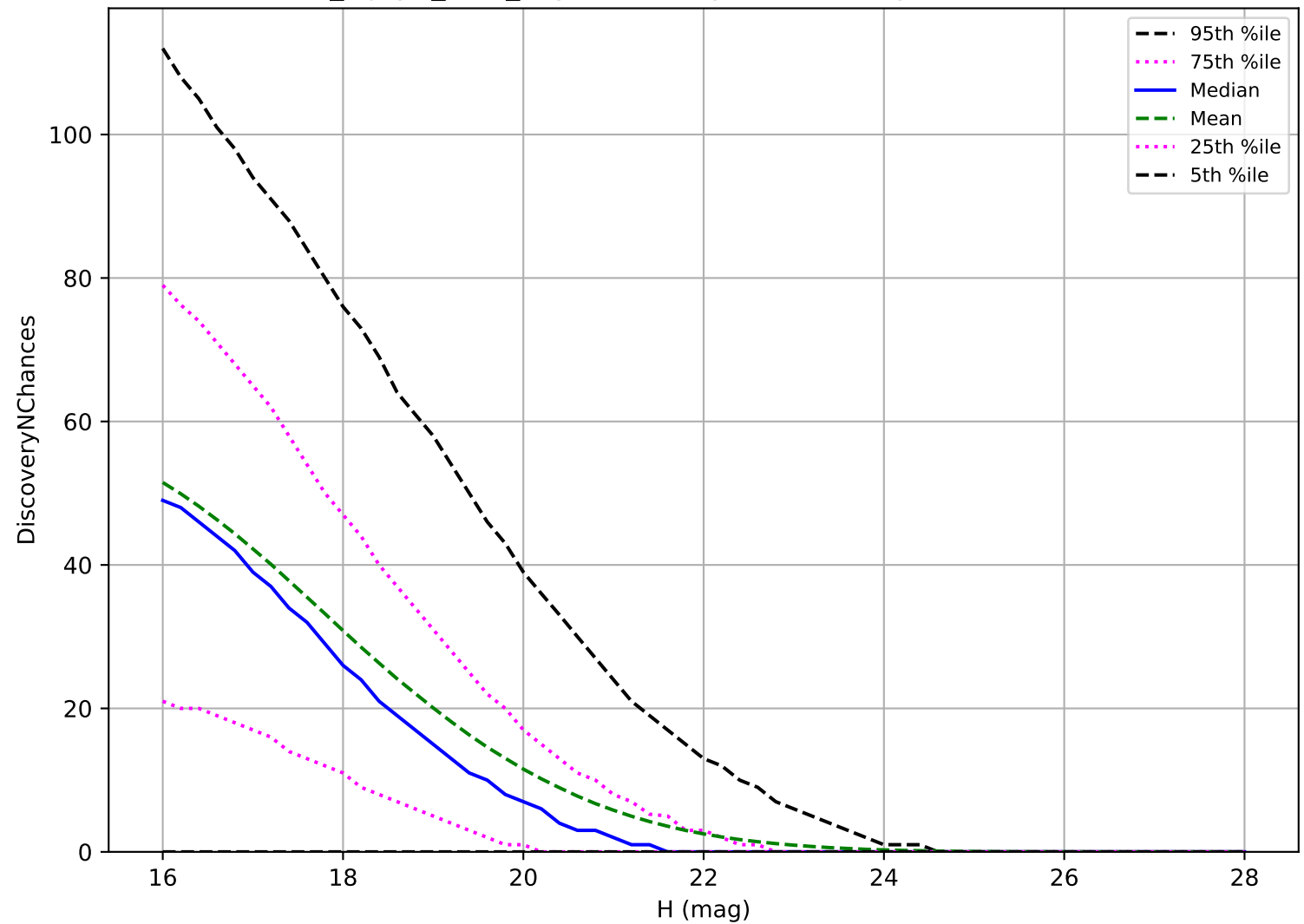
noroll_mjdp0_v3.4_10yrs: NEO 3 pairs in 15 nights detection loss
