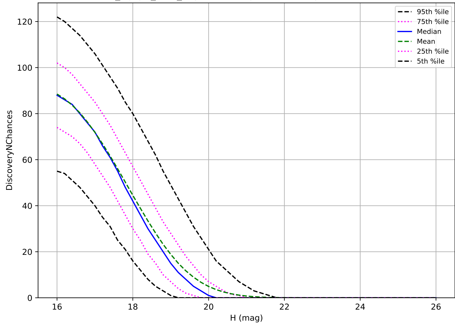
noroll_mjdp0_v3.4_10yrs: MBA 3 pairs in 15 nights detection loss
