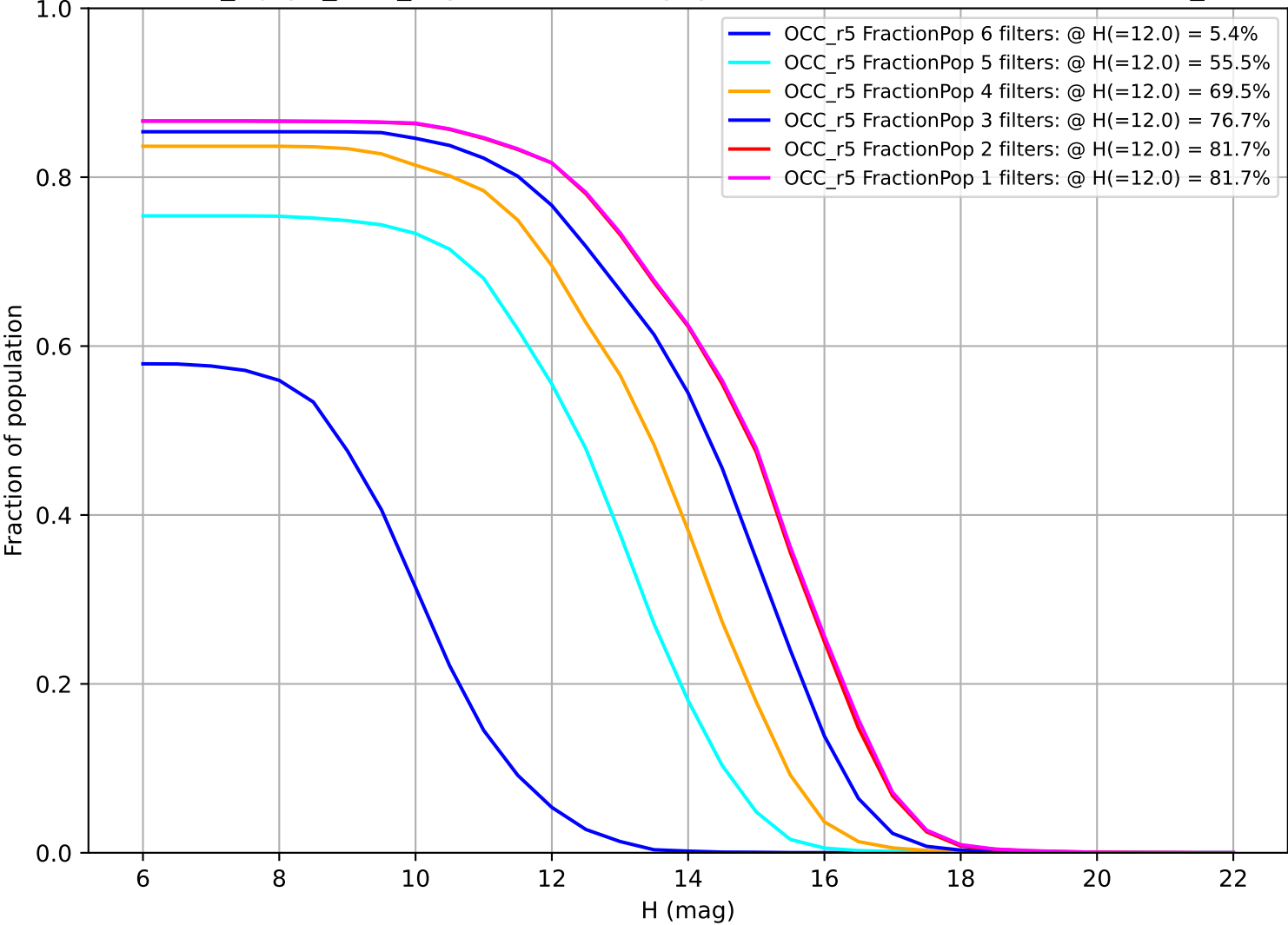
noroll_mjdp0_v3.4_10yrs: Fraction of population with colors in X filters OCC_r5
