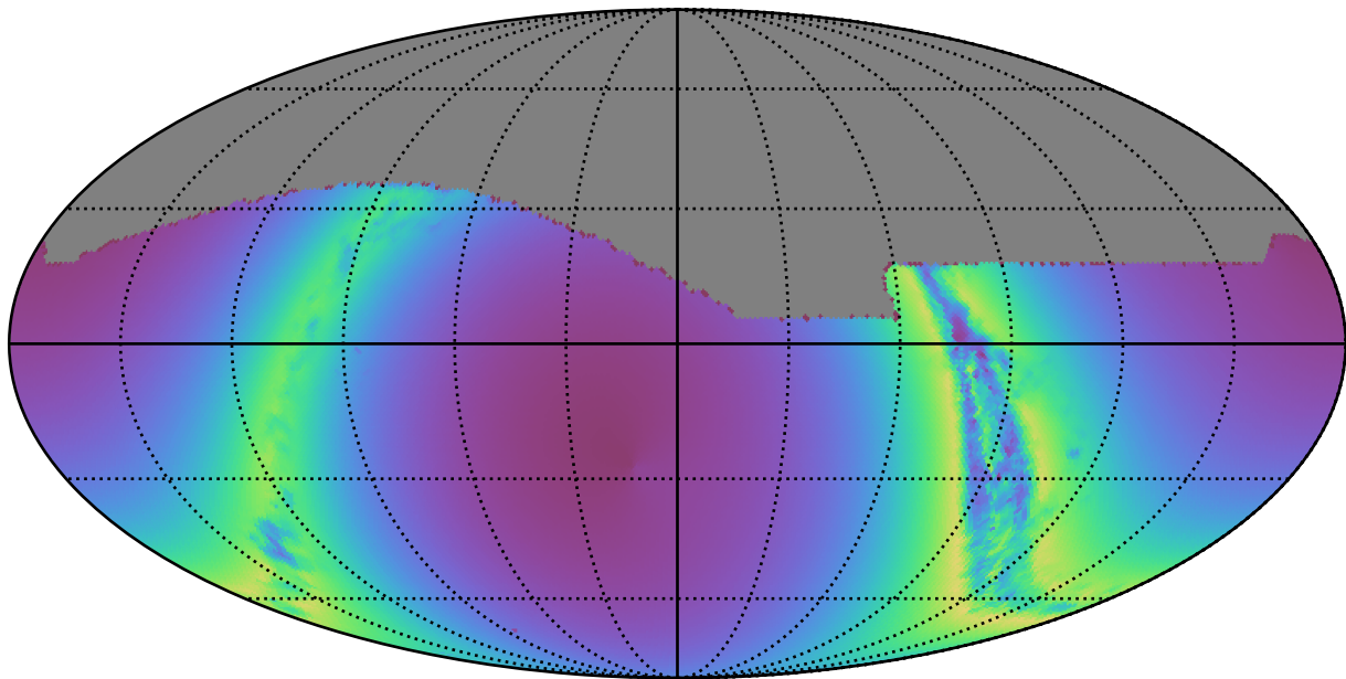
noroll_mjdp0_v3.4_10yrs : young_stars
