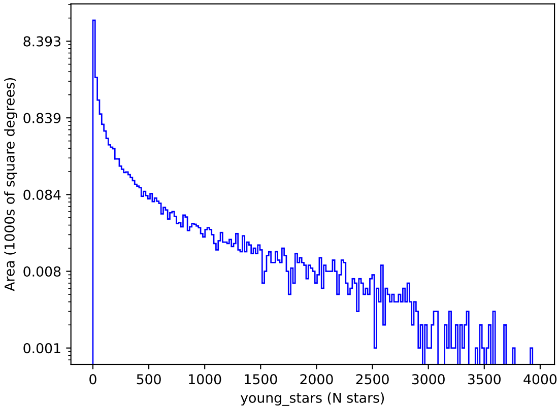
noroll_mjdp0_v3.4_10yrs : young_stars
