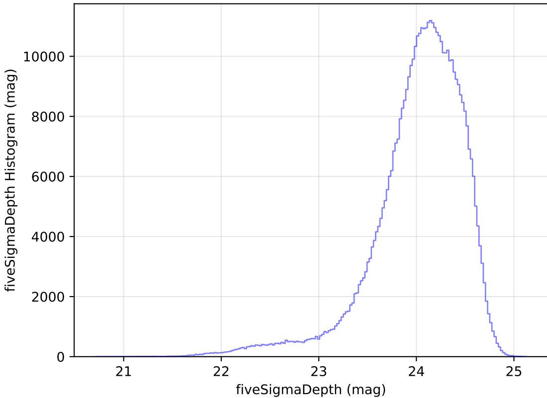
noroll_mjdp0_v3.4_10yrs r: fiveSigmaDepth Histogram
