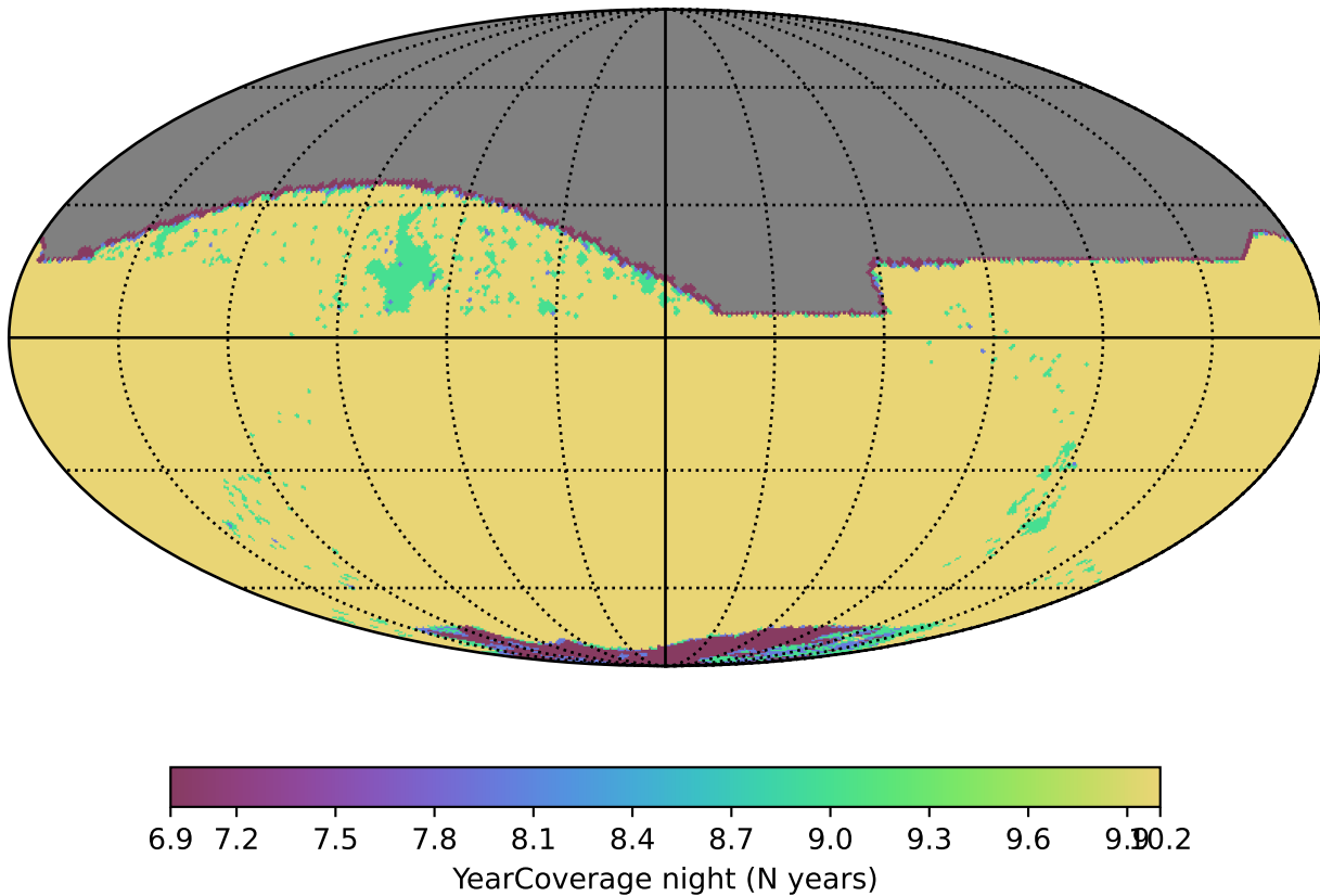
noroll_mjdp0_v3.4_10yrs z band: YearCoverage night
