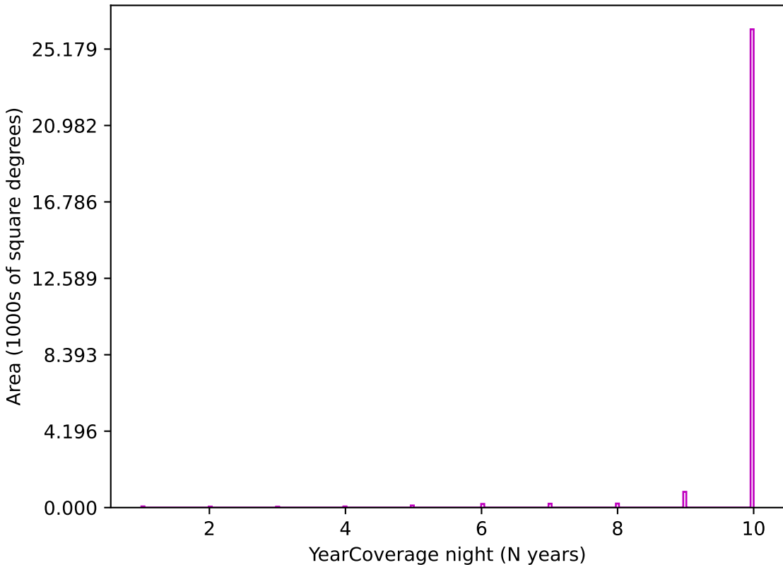
noroll_mjdp0_v3.4_10yrs z band: YearCoverage night
