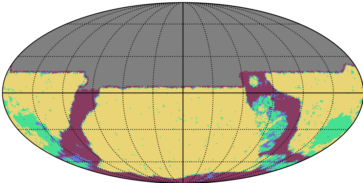
noroll_mjdp0_v3.4_10yrs u band: YearCoverage night
