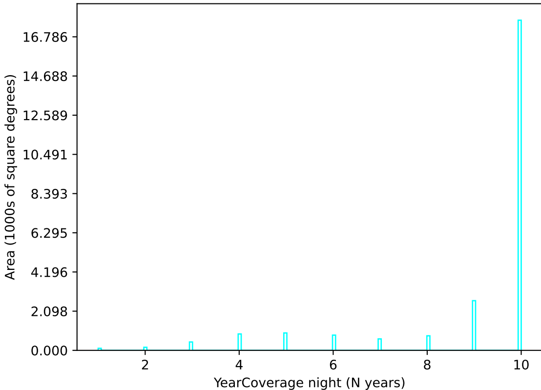
noroll_mjdp0_v3.4_10yrs u band: YearCoverage night
