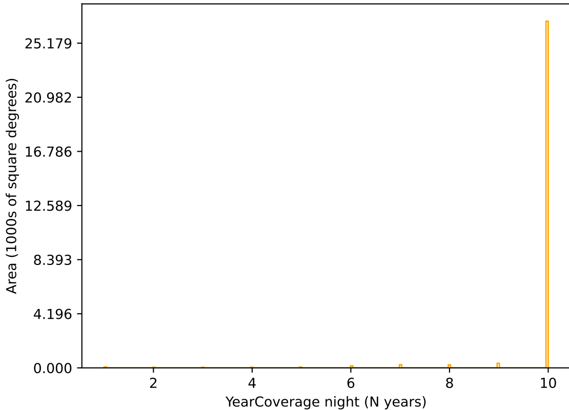
noroll_mjdp0_v3.4_10yrs r band: YearCoverage night
