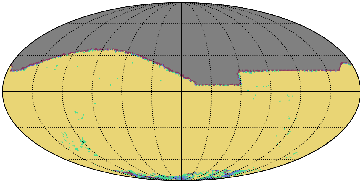
noroll_mjdp0_v3.4_10yrs i band: YearCoverage night
