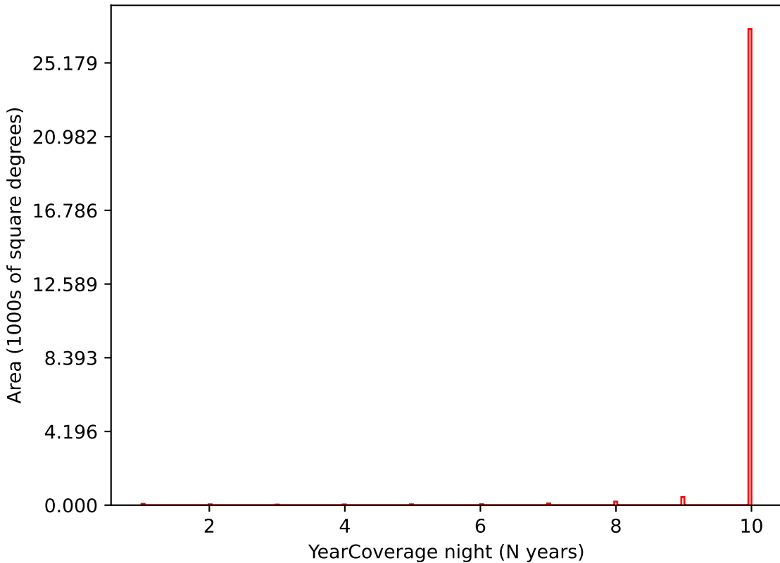
noroll_mjdp0_v3.4_10yrs i band: YearCoverage night
