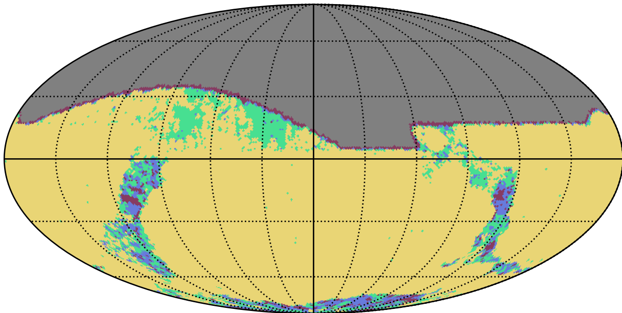
noroll_mjdp0_v3.4_10yrs g band: YearCoverage night
