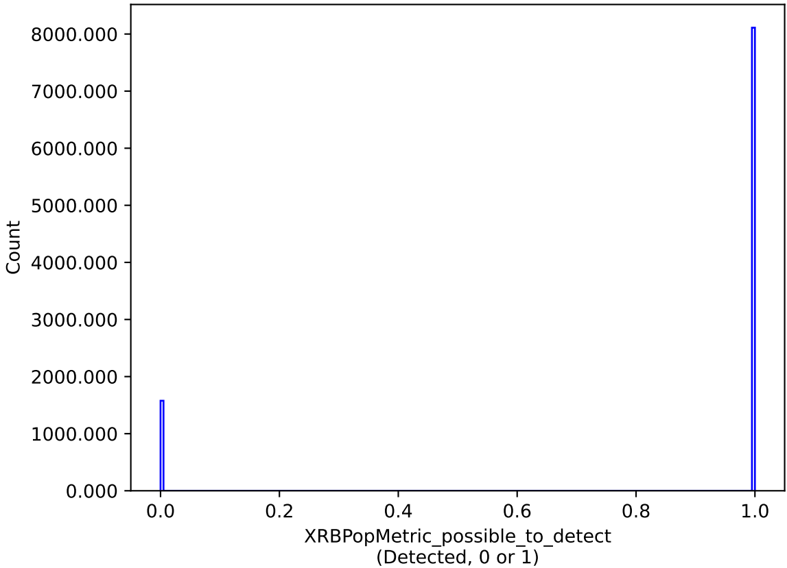
noroll_mjdp0_v3.4_10yrs : XRBPoMetric_possible_to_detect
