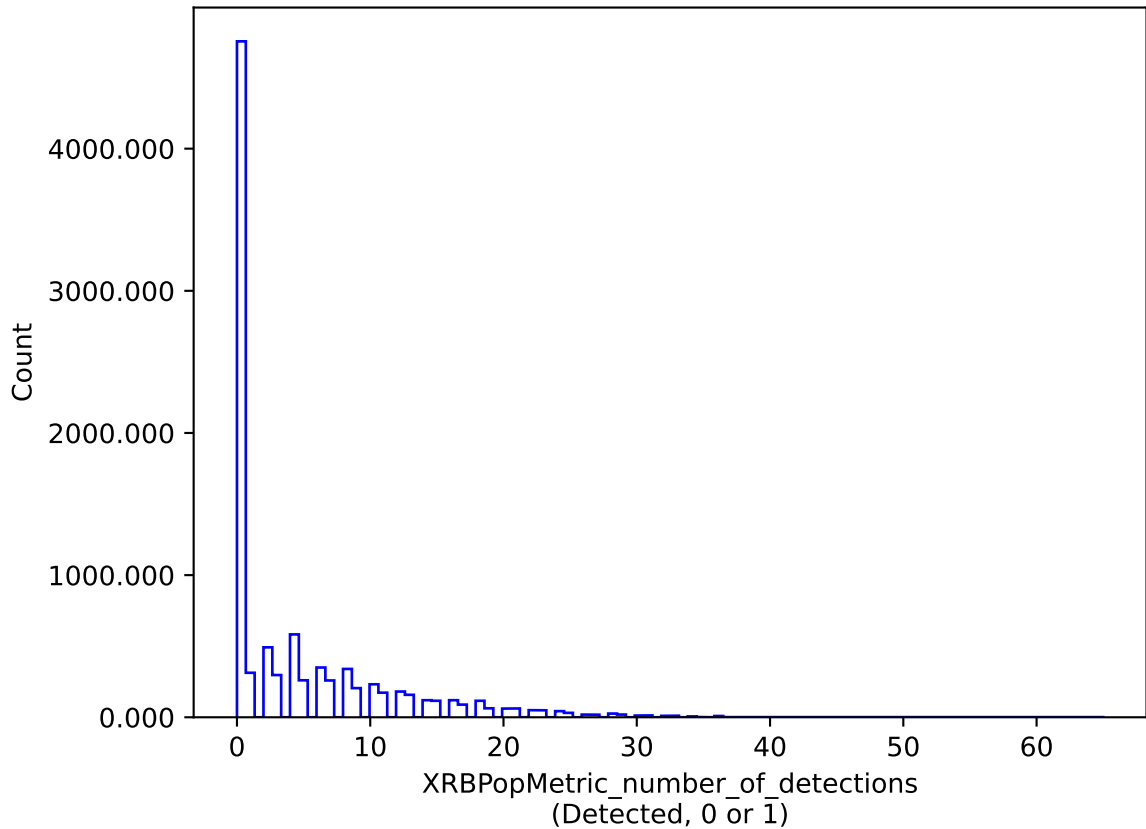
noroll_mjdp0_v3.4_10yrs : XRBPopMetric_number_of_detections
