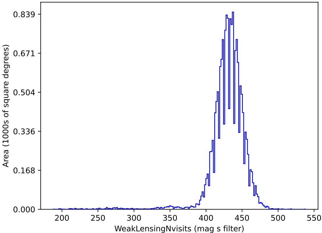
noroll_mjdp0_v3.4_10yrs gri band non-DD: WeakLensingNvisits
