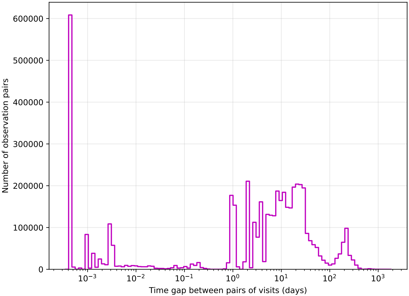
noroll_mjdp0_v3.4_10yrs z band: Tgaps observationStartMJD
