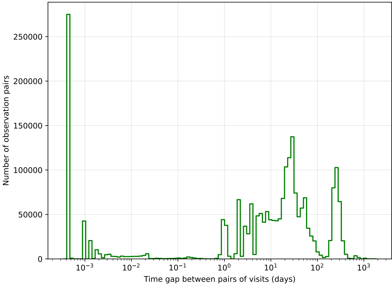
noroll_mjdp0_v3.4_10yrs g band: Tgaps observationStartMJD
