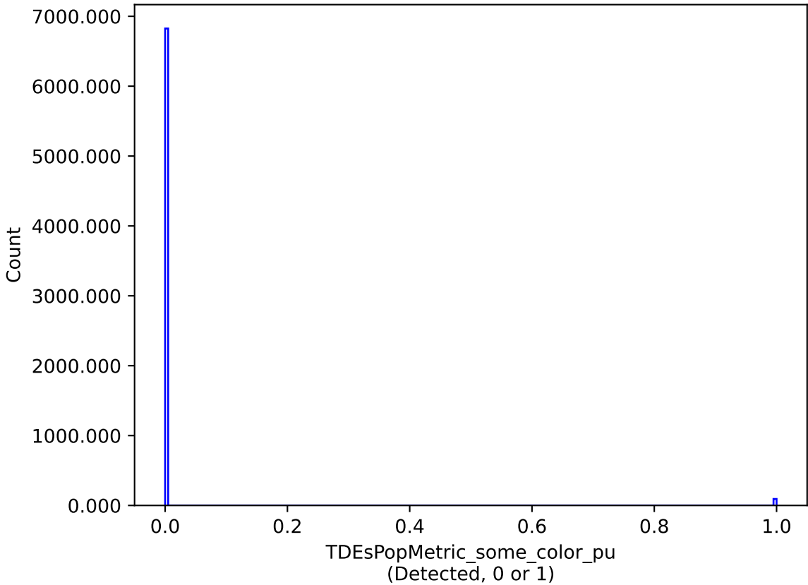
noroll_mjdp0_v3.4_10yrs : TDEsPopMetric_some_color_pu
