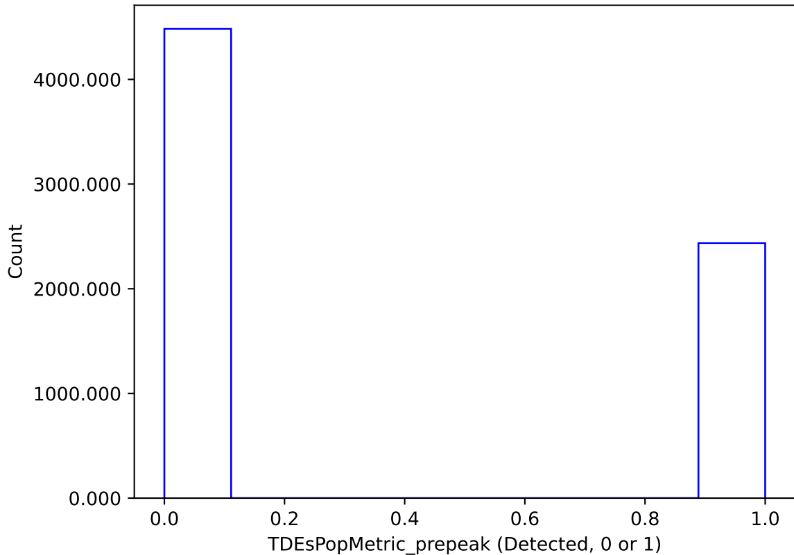
noroll_mjdp0_v3.4_10yrs : TDEsPopMetric_prepeak
