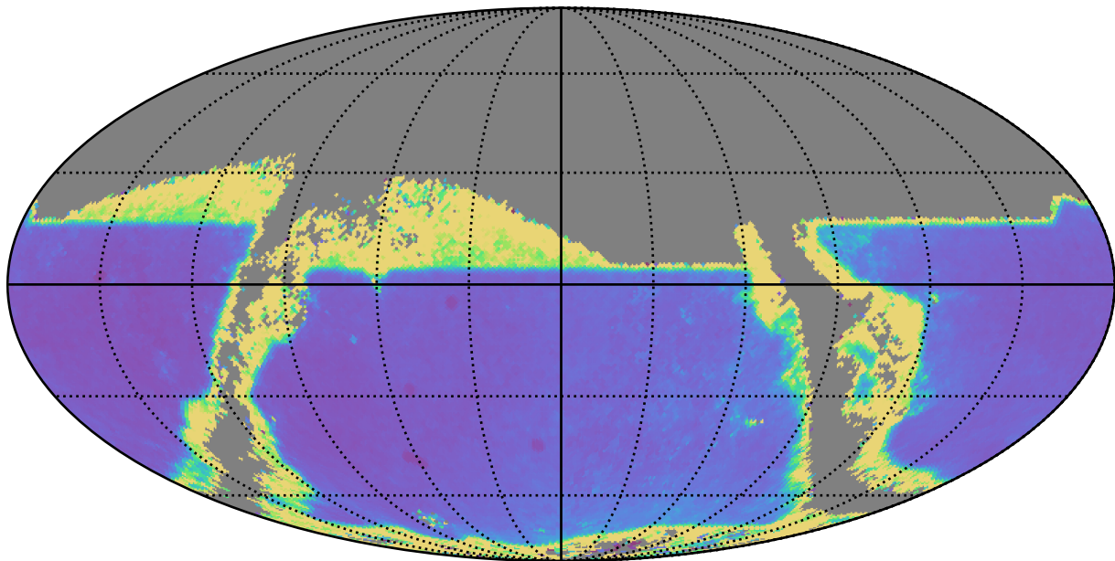
noroll_mjdp0_v3.4_10yrs : TDC_cadence
