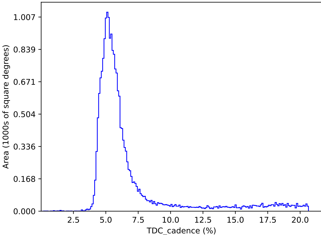
noroll_mjdp0_v3.4_10yrs : TDC_cadence
