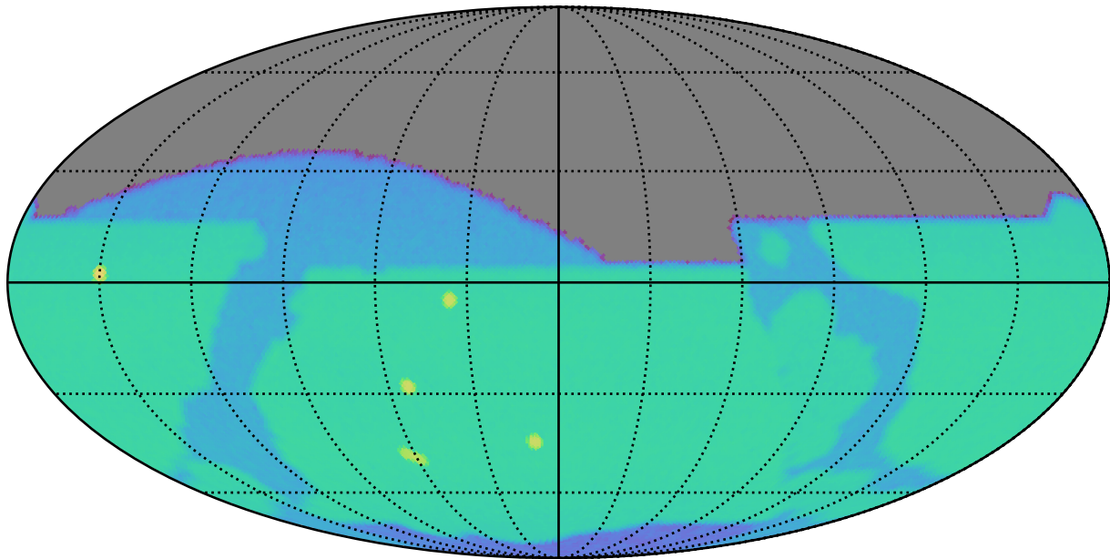
noroll_mjdp0_v3.4_10yrs z: SurfaceBrightLimit
