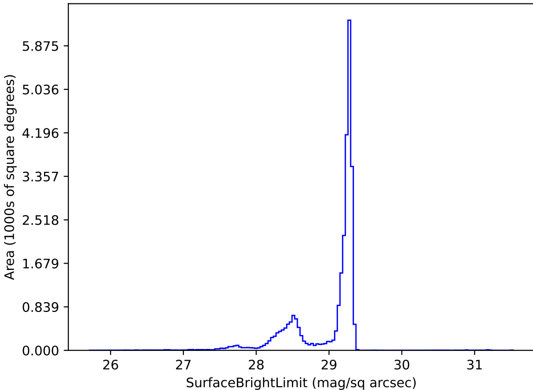
noroll_mjdp0_v3.4_10yrs z: SurfaceBrightLimit
