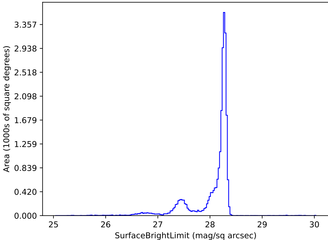
noroll_mjdp0_v3.4_10yrs y: SurfaceBrightLimit
