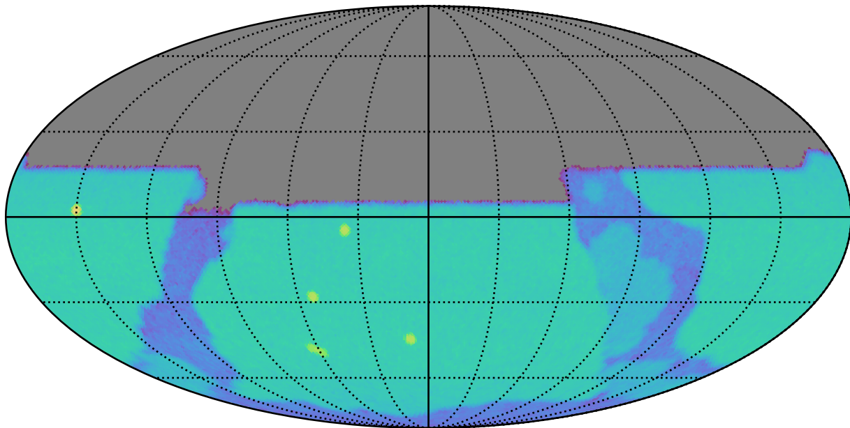
noroll_mjdp0_v3.4_10yrs u: SurfaceBrightLimit
