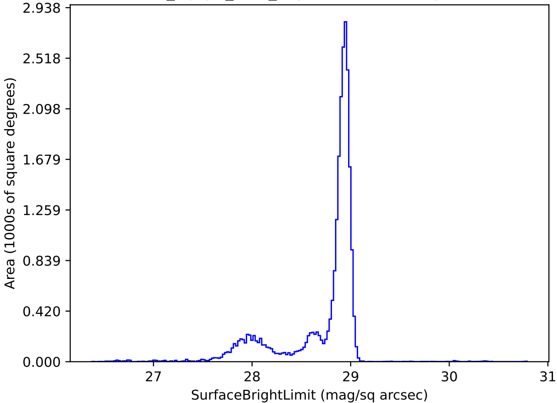
noroll_mjdp0_v3.4_10yrs u: SurfaceBrightLimit
