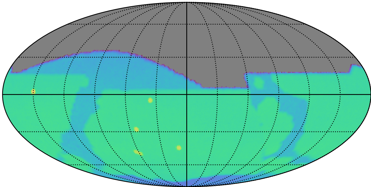
noroll_mjdp0_v3.4_10yrs r: SurfaceBrightLimit
