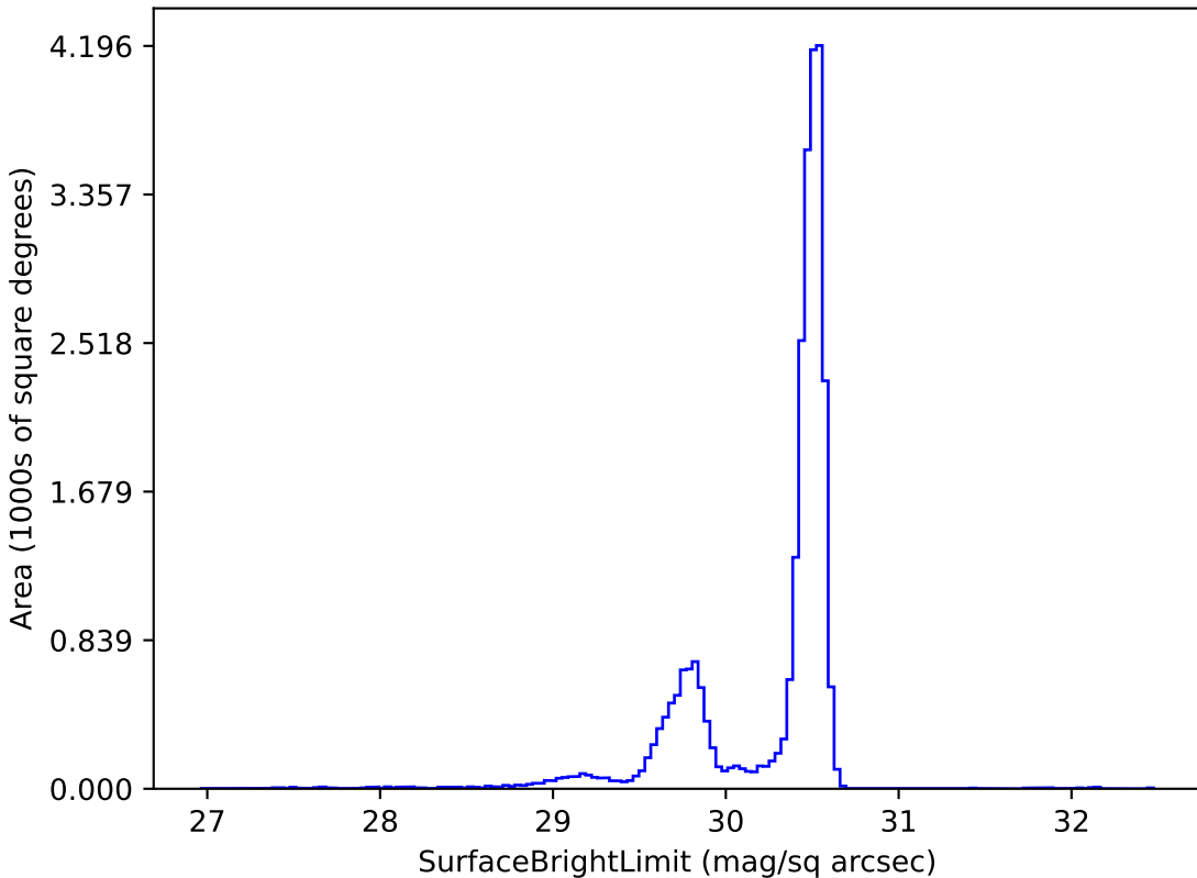
noroll_mjdp0_v3.4_10yrs r: SurfaceBrightLimit
