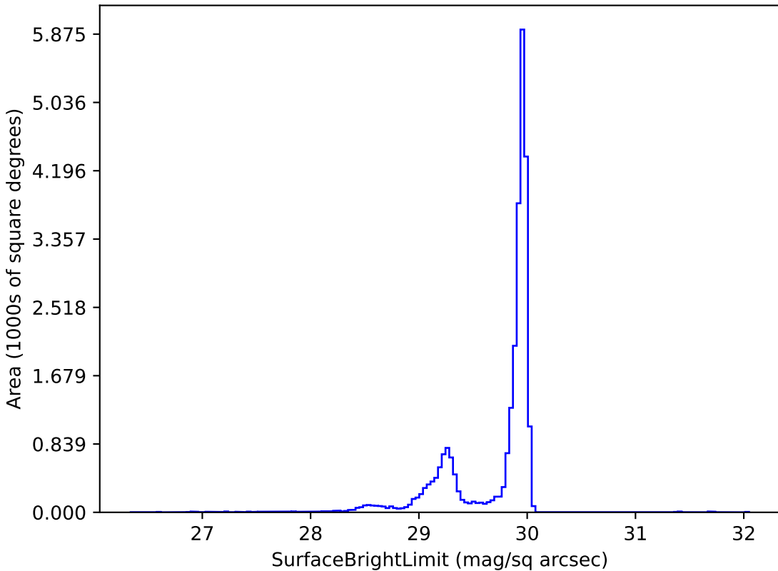
noroll_mjdp0_v3.4_10yrs i: SurfaceBrightLimit
