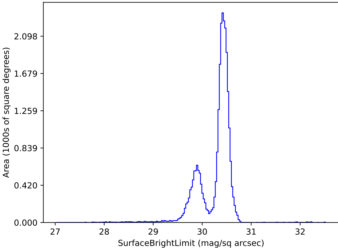
noroll_mjdp0_v3.4_10yrs g: SurfaceBrightLimit
