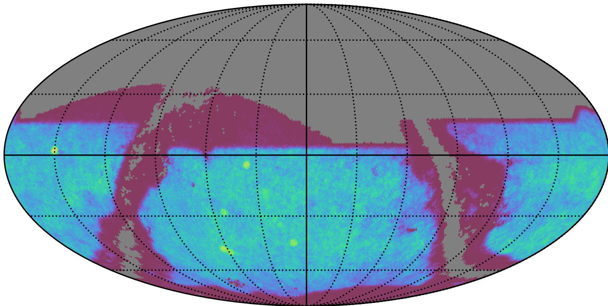
noroll_mjdp0_v3.4_10yrs : SNSLMetric
