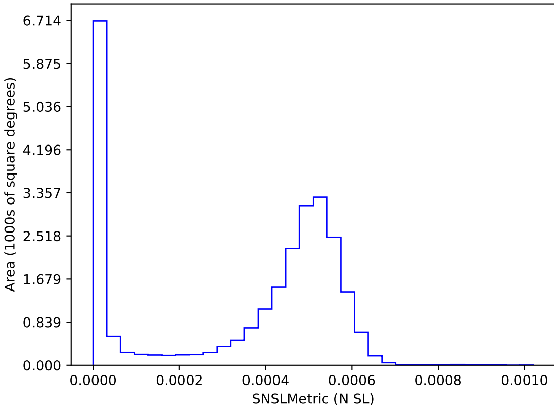
noroll_mjdp0_v3.4_10yrs : SNSLMetric
