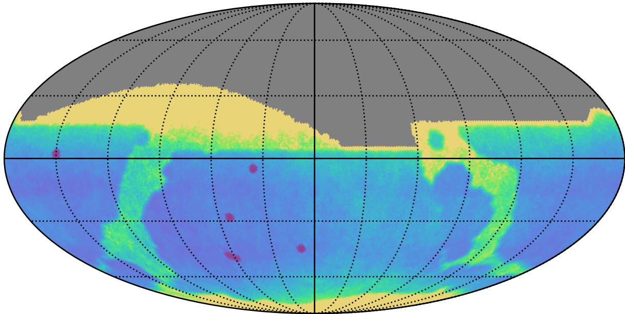
noroll_mjdp0_v3.4_10yrs : Proper Motion Uncert @ 24.0
