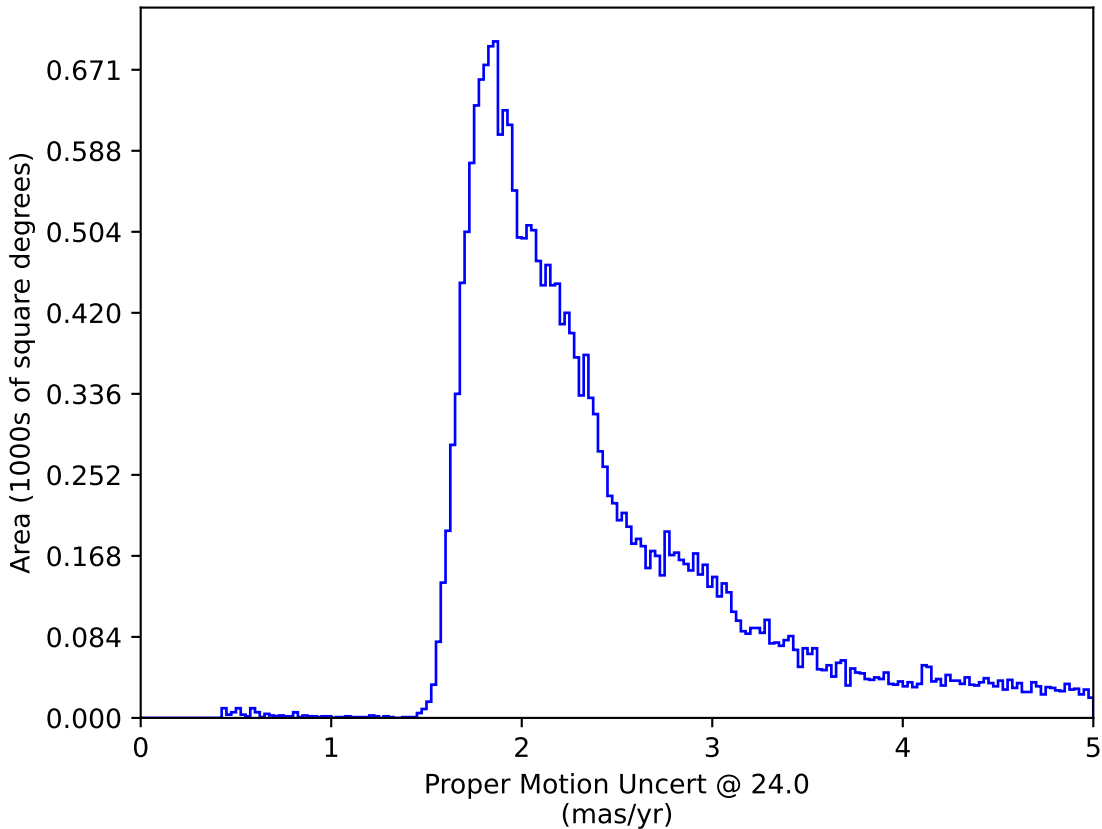
noroll_mjdp0_v3.4_10yrs : Proper Motion Uncert @ 24.0
