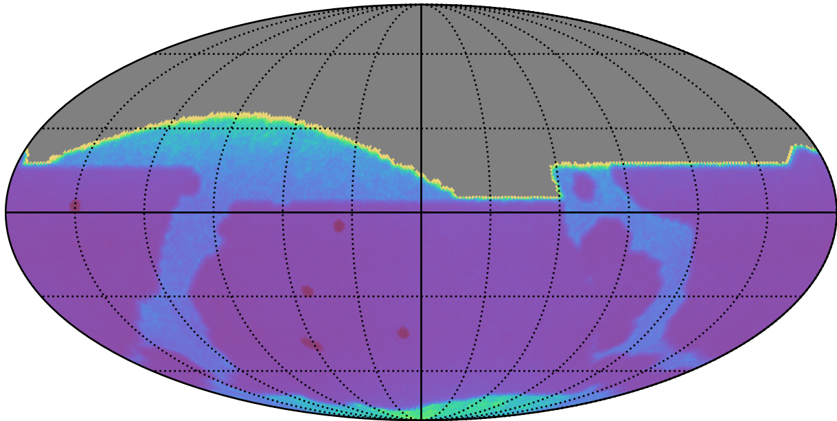
noroll_mjdp0_v3.4_10yrs : Proper Motion Uncert @ 20.5
