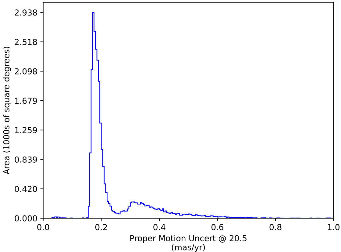
noroll_mjdp0_v3.4_10yrs : Proper Motion Uncert @ 20.5
