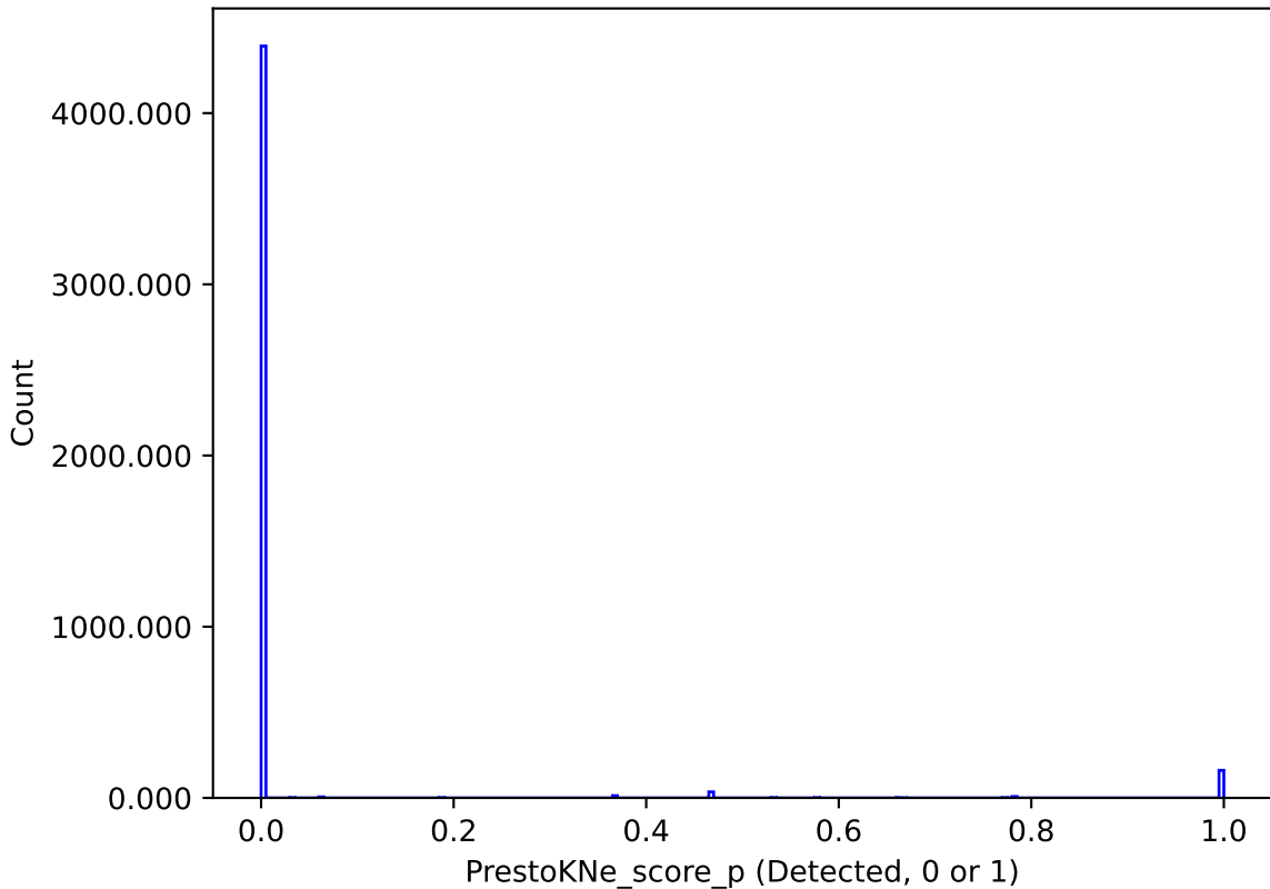
noroll_mjdp0_v3.4_10yrs : PrestoKNe_score_p
