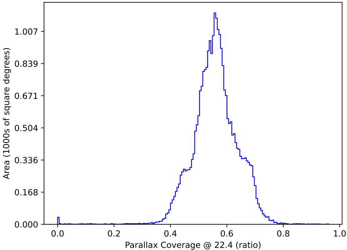
noroll_mjdp0_v3.4_10yrs : Parallax Coverage @ 22.4
