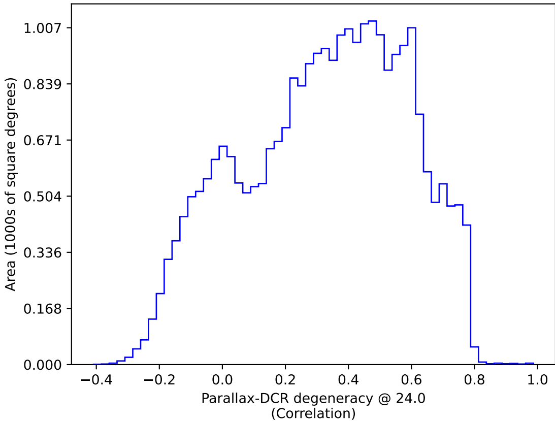
noroll_mjdp0_v3.4_10yrs : Parallax-DCR degeneracy @ 24.0
