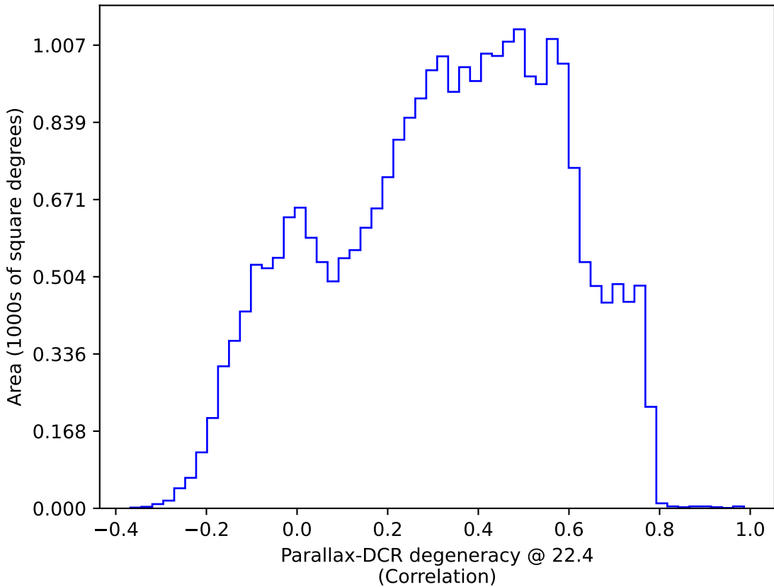
noroll_mjdp0_v3.4_10yrs : Parallax-DCR degeneracy @ 22.4
