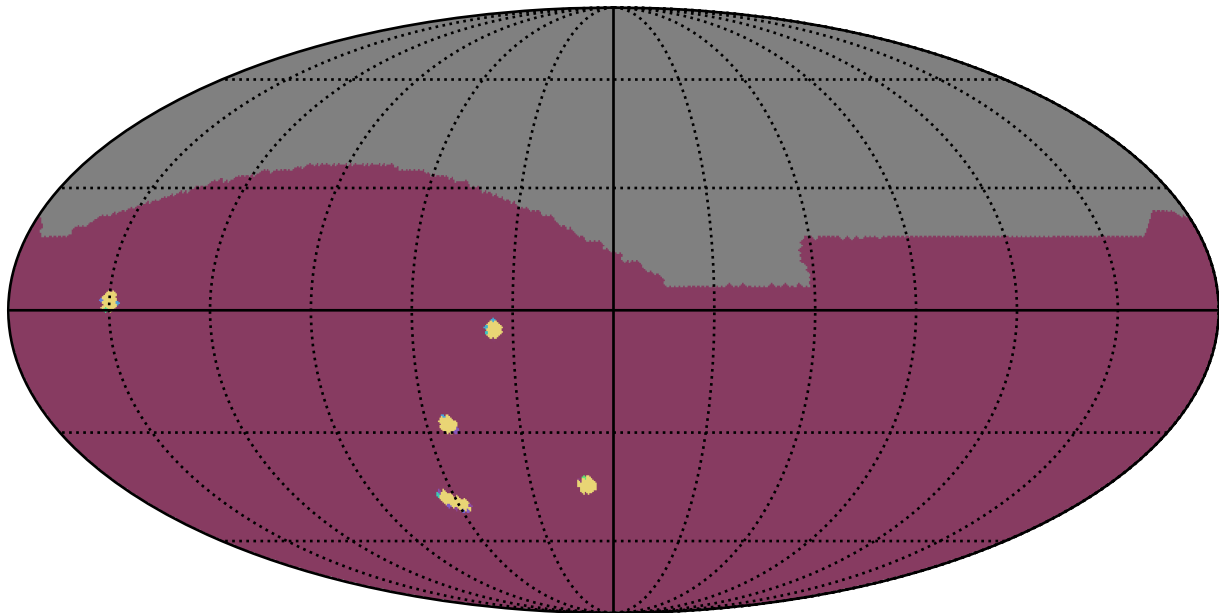
noroll_mjdp0_v3.4_10yrs : NumberOfQuickRevisits
