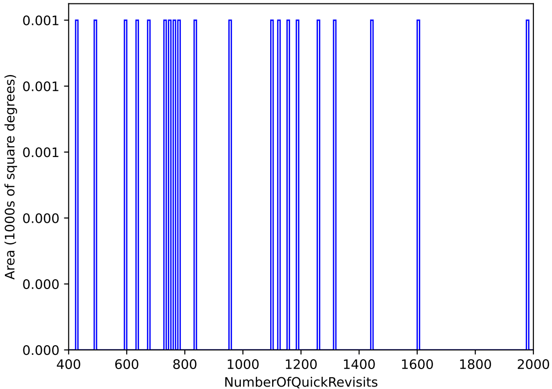
noroll_mjdp0_v3.4_10yrs : NumberOfQuickRevisits
