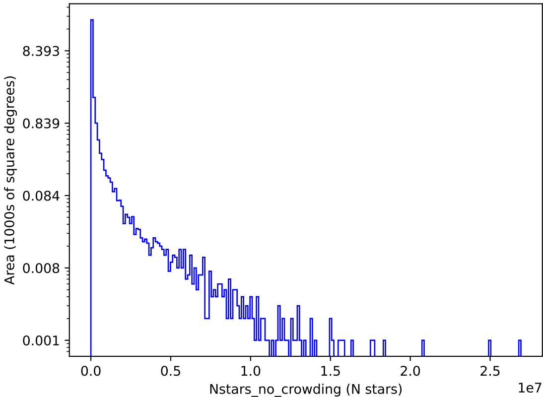
noroll_mjdp0_v3.4_10yrs z: Nstars_no_crowding
