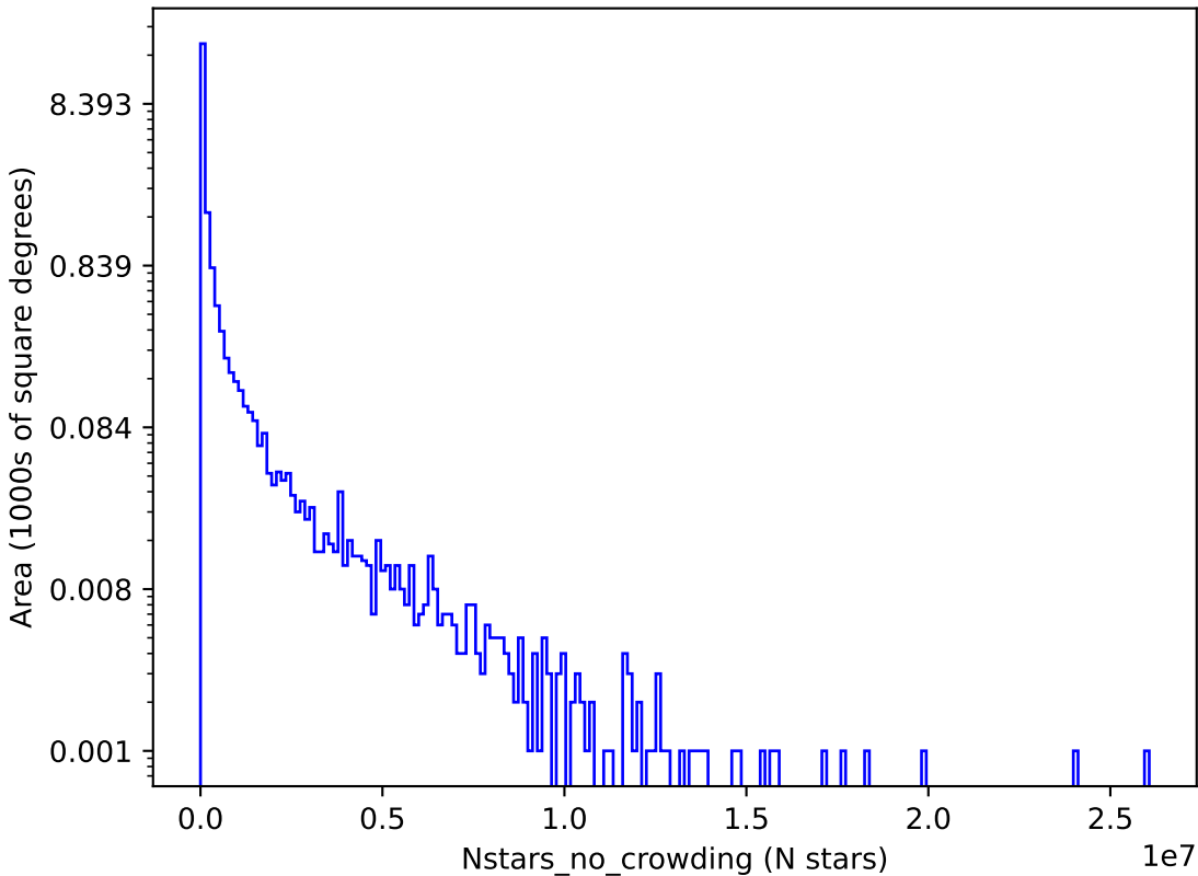
noroll_mjdp0_v3.4_10yrs y: Nstars_no_crowding
