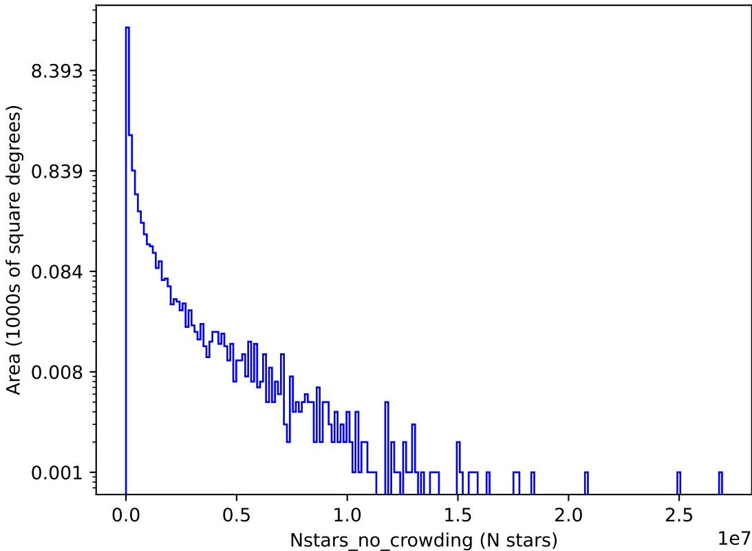
noroll_mjdp0_v3.4_10yrs i: Nstars_no_crowding
