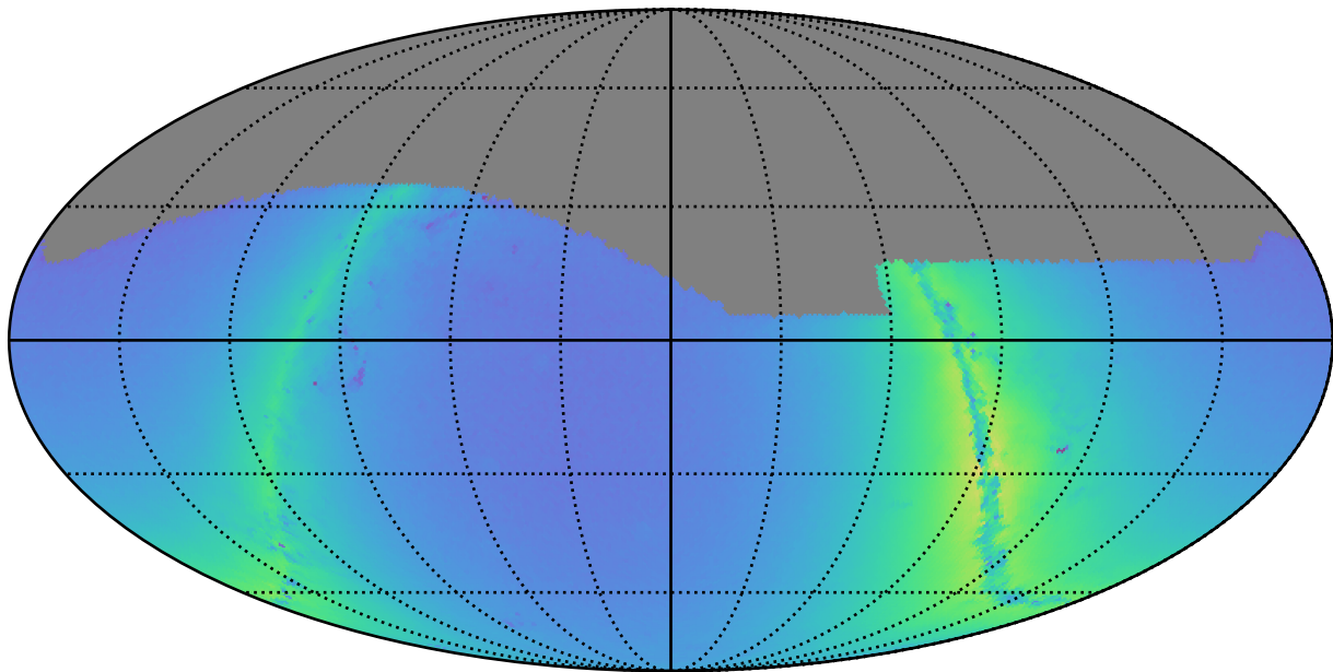
noroll_mjdp0_v3.4_10yrs g: Nstars_no_crowding
