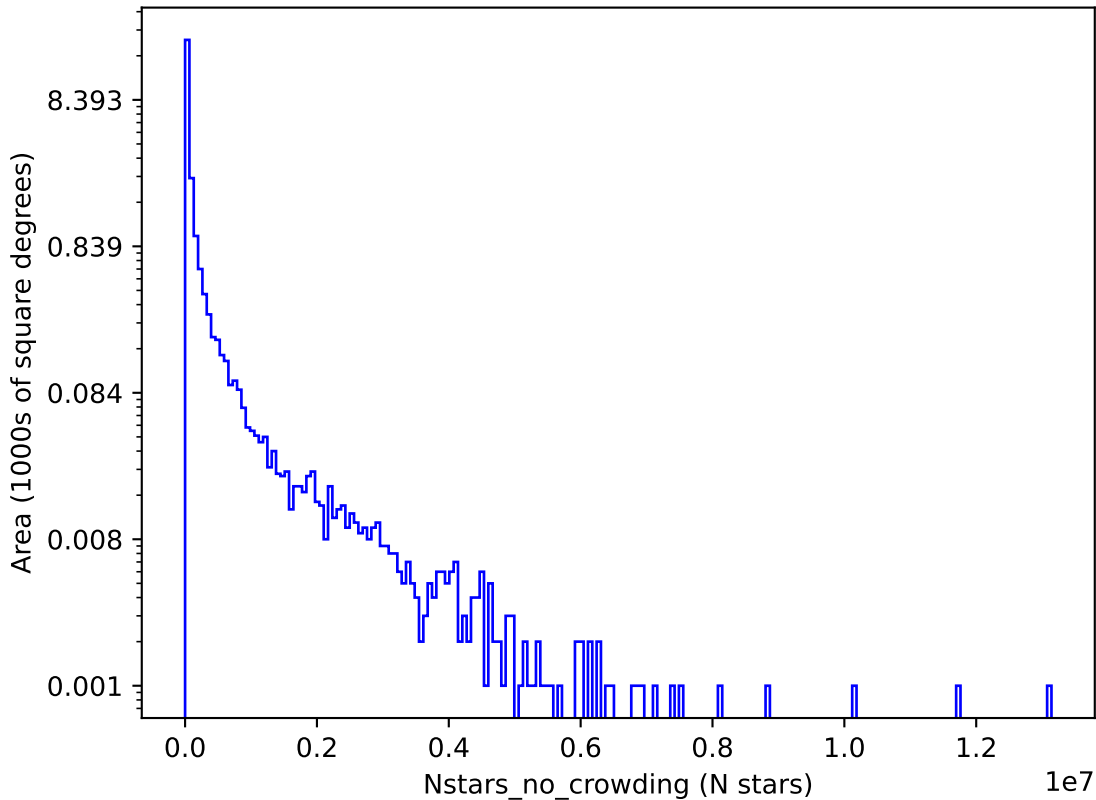
noroll_mjdp0_v3.4_10yrs g: Nstars_no_crowding
