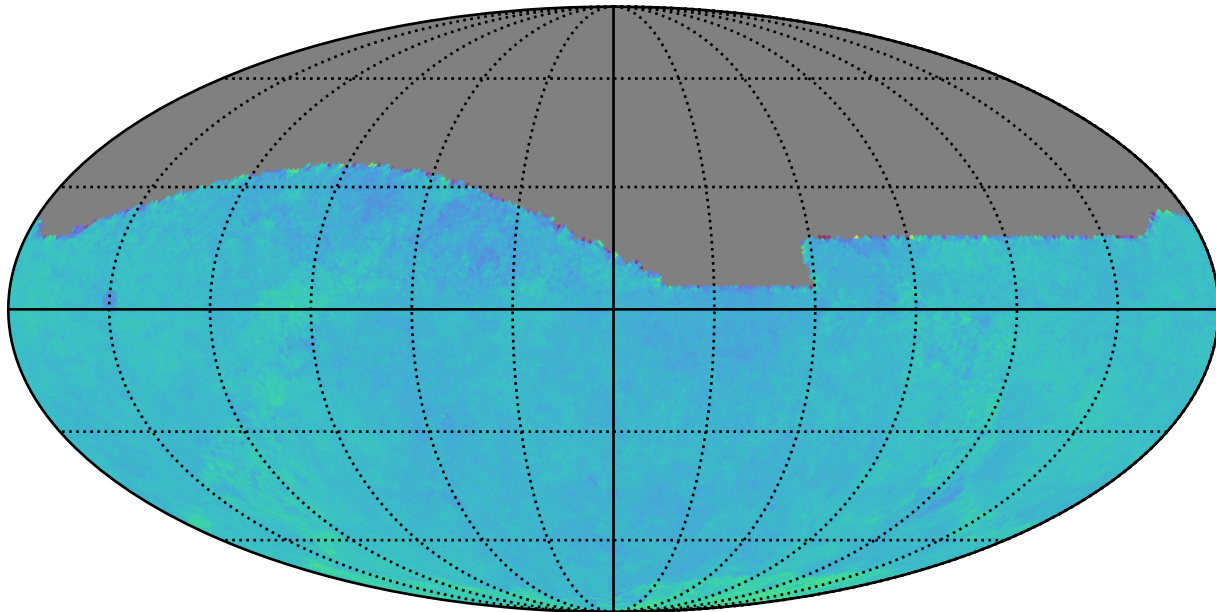
noroll_mjdp0_v3.4_10yrs : Normalized Proper Motion Uncert @ 24.0
